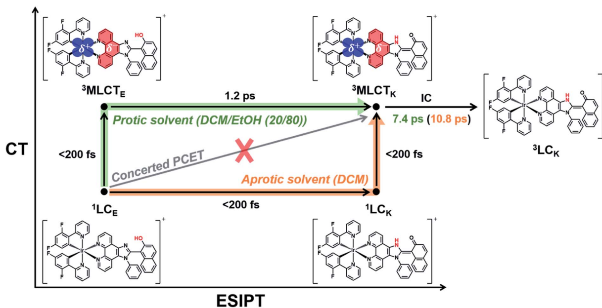
Fig. 5 Excited-state relaxation dynamics for PCET in Ir-PIPn in an aprotic solvent and a protic solvent in the axes of the CT and ESIPT. Reaction pathways in an aprotic solvent and a protic solvent are indicated by orange and green arrows, respectively. The subscripts E and K refer to the enol and keto forms, respectively. In the CT axis, the charge density difference shows the change in the charge distribution induced by the MLCT transition. The blue- and red-marked regions indicate the decrease ( \delta^+ ) and increase ( \delta^- ) in negative charge densities, respectively.
