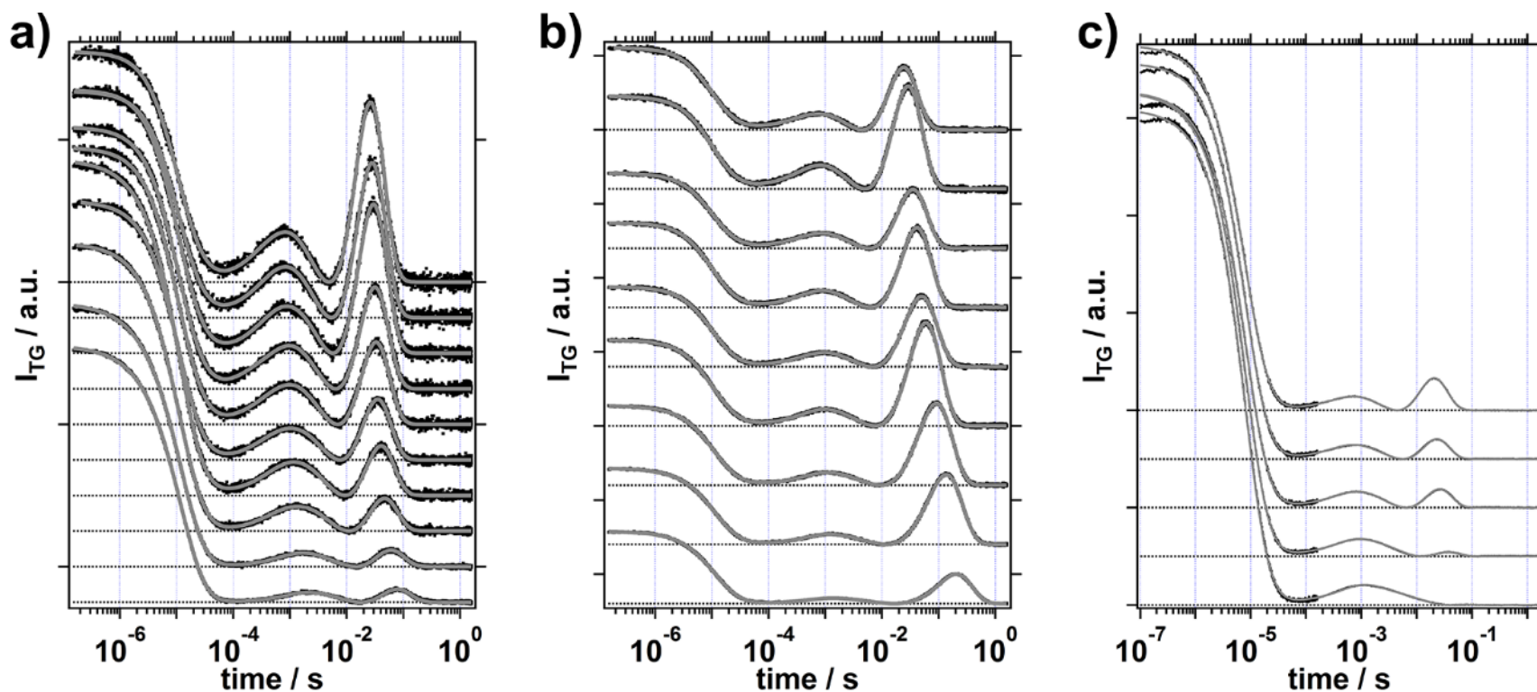
Fig. S8. a) TG signals after photoexcitation of PYP at q^2 = 3.76 \times 10^{11} \text{ m}^{-2} as a function of the concentration of EG. From top to bottom, the concentration of PEG EG are 0, 2, 4, 6, 8, 10, 15, 20, 30 and 40% (v/v). b) TG signals after photoexcitation of PYP at q^2 = 4.27 \times 10^{11} \text{ m}^{-2} as a function of the concentration of PEG 8000. From top to bottom, the concentration of PEG 8000 are 0, 2, 5, 7, 9, 12, 17, 23 and 28% (v/v). c) TG signals after photoexcitation of PYP at q^2 = 4.4 \times 10^{11} \text{ m}^{-2} as a function of the concentration of Dextran 40. From top to bottom, the concentration of Dextran 40 are 0, 2, 4, and 9% (v/v). Experimental signals (black) and theoretical signals (gray) calculated by using Eq. (1) are shown.
