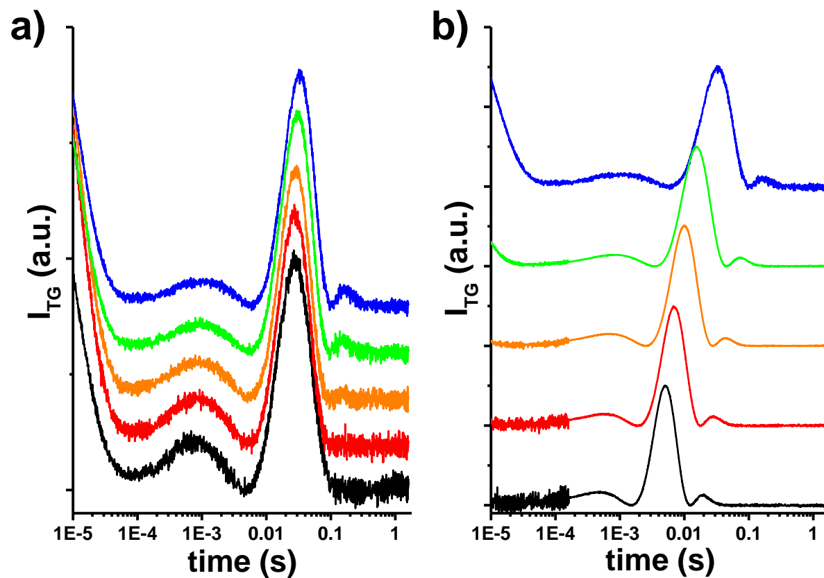
Fig. S10. TG signals. a) TG signals after photoexcitation of PYP at q^2 = 0.37 \times 10^{12} \text{ m}^{-2} as a function of the concentration of BSA. From bottom to top, the concentrations of BSA are 0, 4, 7, 11, and 14% v/v. b) TG signals after photoexcitation of PYP with 200 g/L BSA at various q^2 ranges (From bottom to top, q^2 = 3.85, 2.62, 1.61, 0.93, and 0.37 \times 10^{12} \text{ m}^{-2} )
