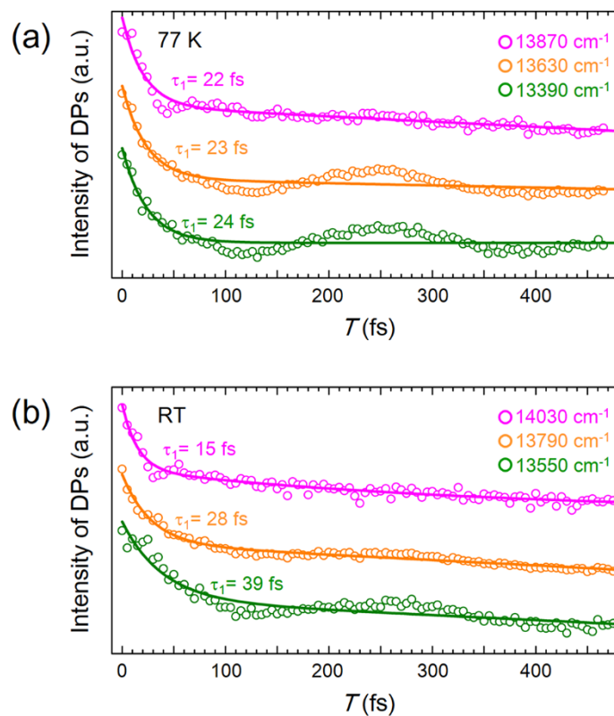
Figure S5. Time traces of the 2D-ES signal amplitude in the population time range up to 480 fs at three selected diagonal points at (a) 77 K (magenta: \omega_\tau = \omega_t = 13870 \text{ cm}^{-1} , orange: \omega_\tau = \omega_t = 13630 \text{ cm}^{-1} , green: \omega_\tau = \omega_t = 13390 \text{ cm}^{-1} ) and (b) RT (magenta: \omega_\tau = \omega_t = 14030 \text{ cm}^{-1} , orange: \omega_\tau = \omega_t = 13790 \text{ cm}^{-1} , green: \omega_\tau = \omega_t = 13550 \text{ cm}^{-1} ).
